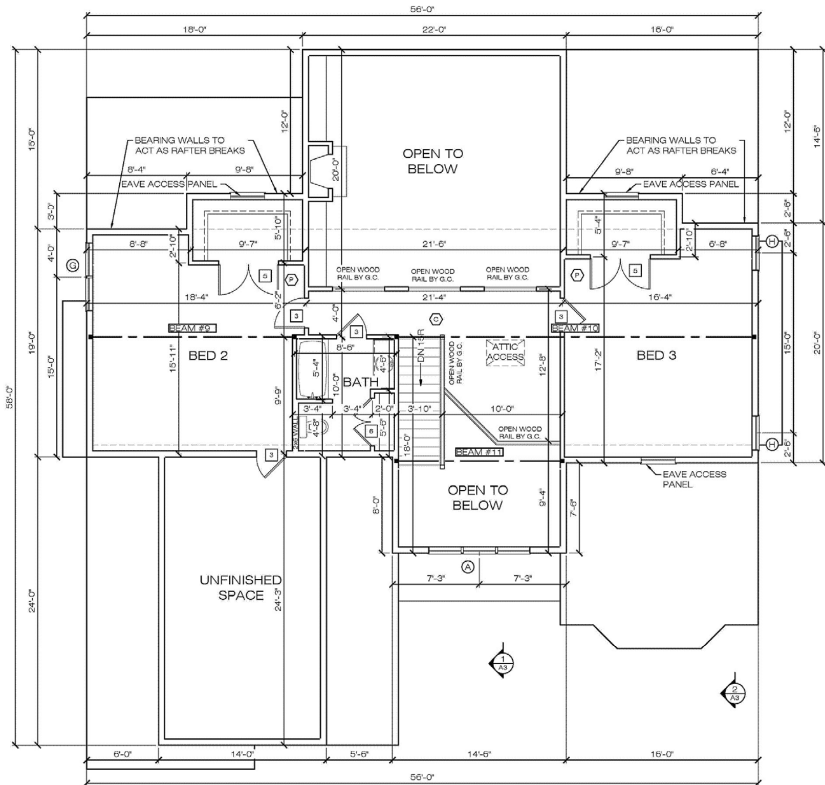
SECOND FLOOR PLAN 1,018 SQ. FT.
